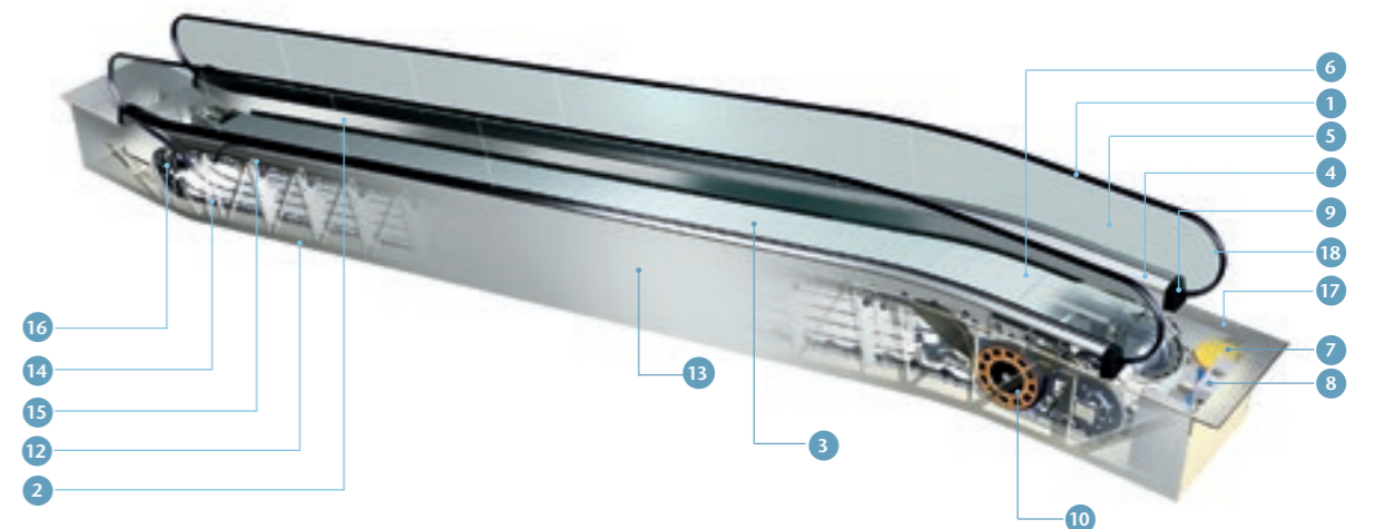
Figure 3.3 Inclined autowalk components
