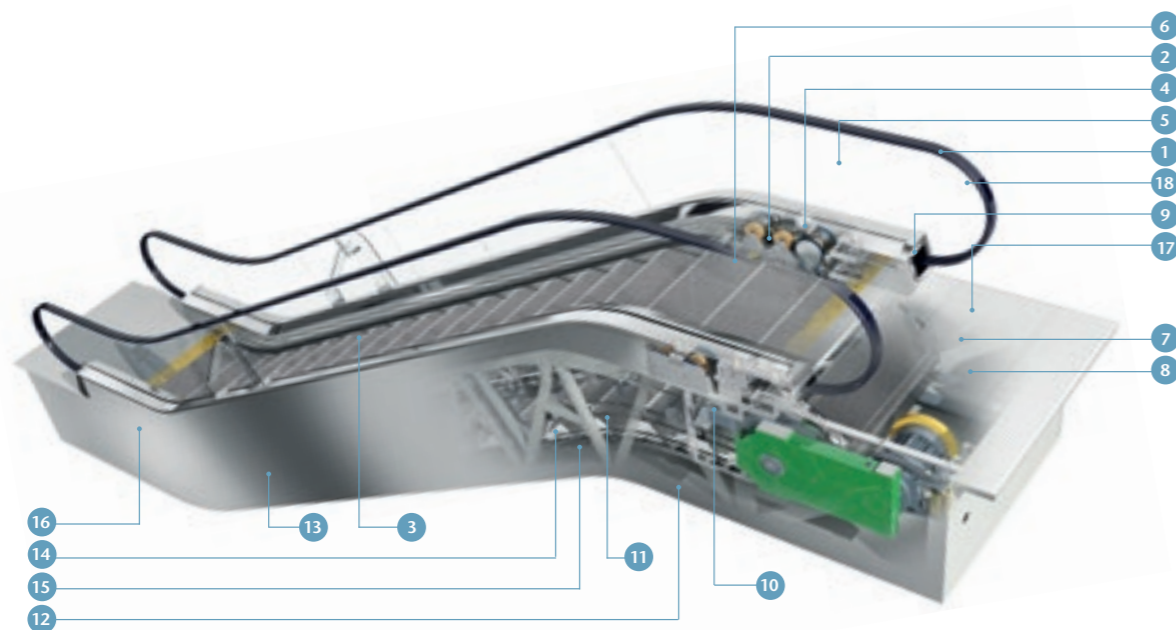
Figure 3.1 Escalator components
