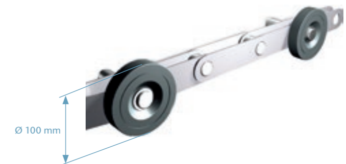
Figure 5.1 Step chain with outside rollers
