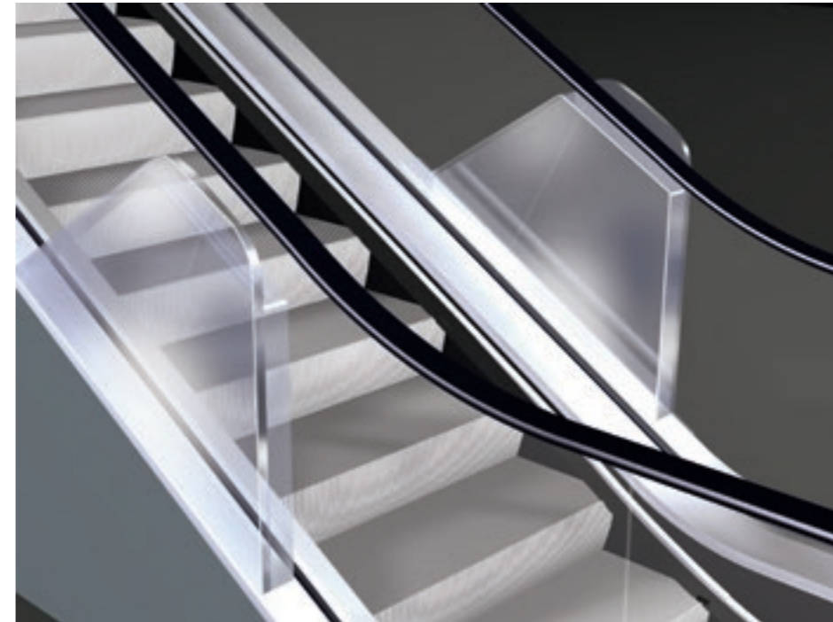
Figure 6.7 Anti-climb device
