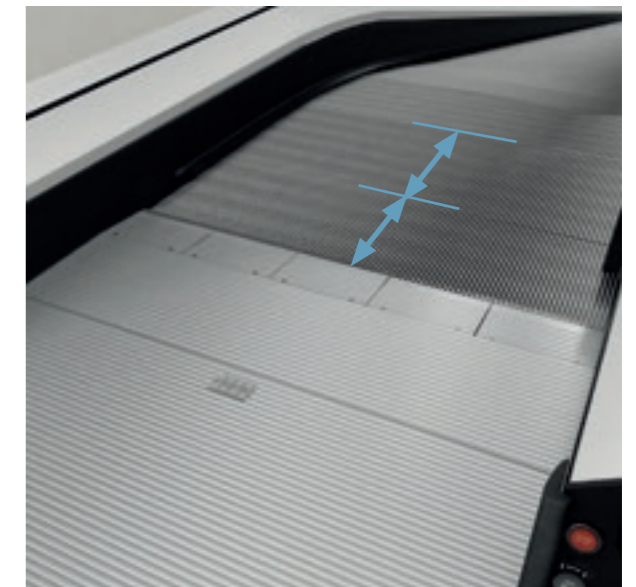
Figure 5.12 The number of horizontal pallets required for inclined autowalks varies with the speed and inclination (one horizontal pallet on the top, two horizontal pallets on the bottom picture).
